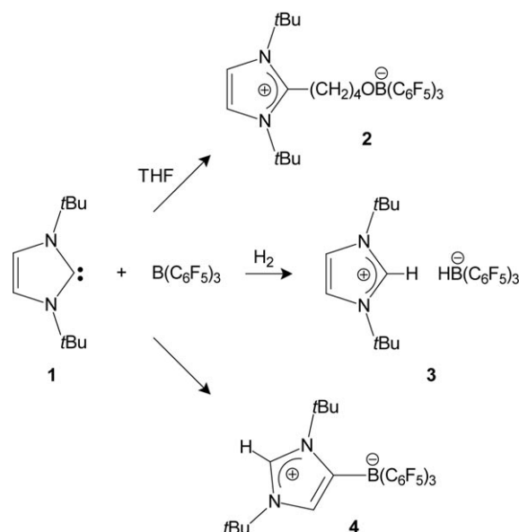
Scheme 1. Reactions of the frustrated Lewis pair (FLP) 1 /B(C 6 F 5 ) 3 .
